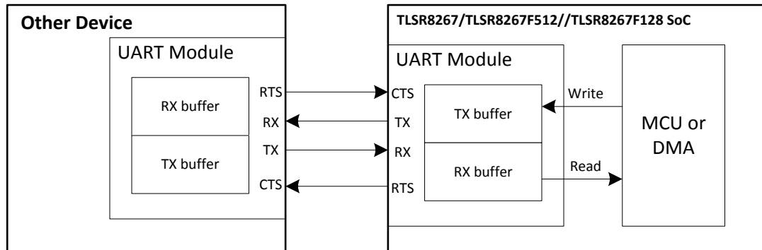
Figure 7- 9 UART communication
