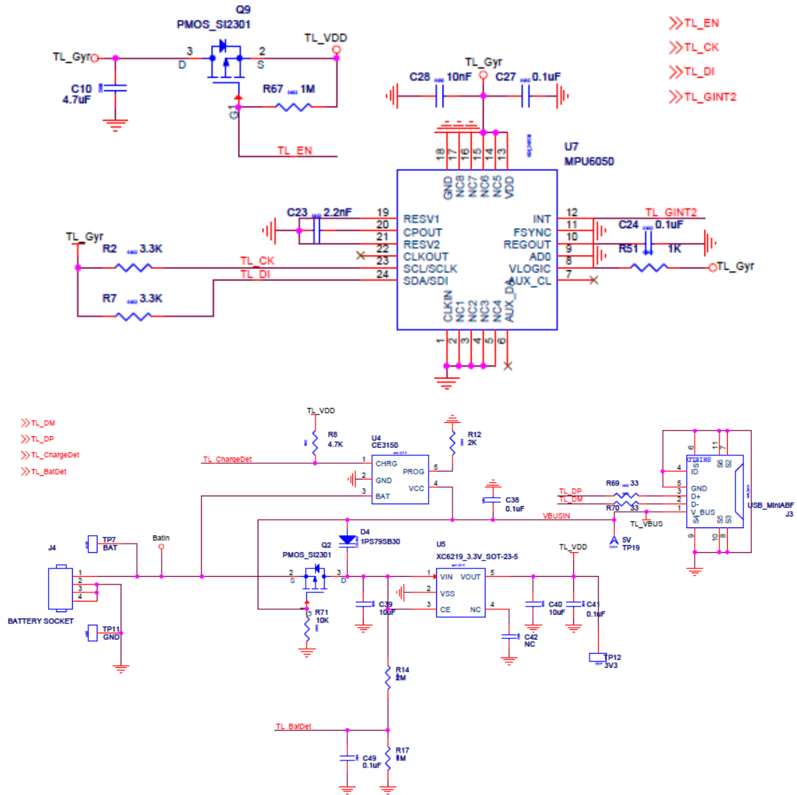
Figure 14- 1Schematic for the TSLR8267ET48
