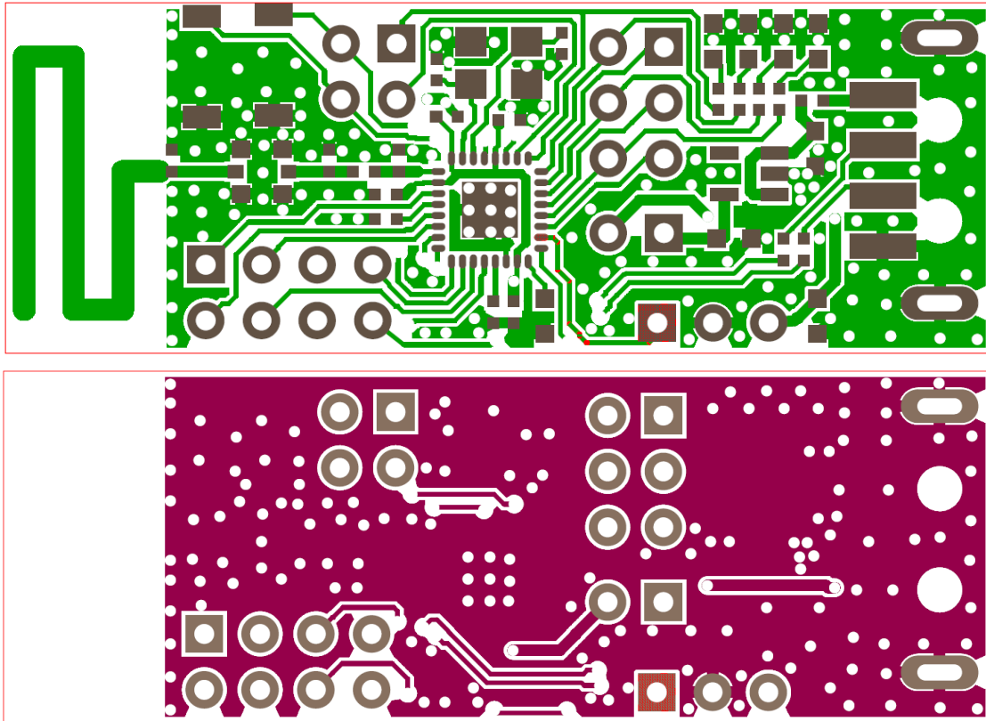
Figure 14- 6 Layout for the TLSR8267F512ET32
