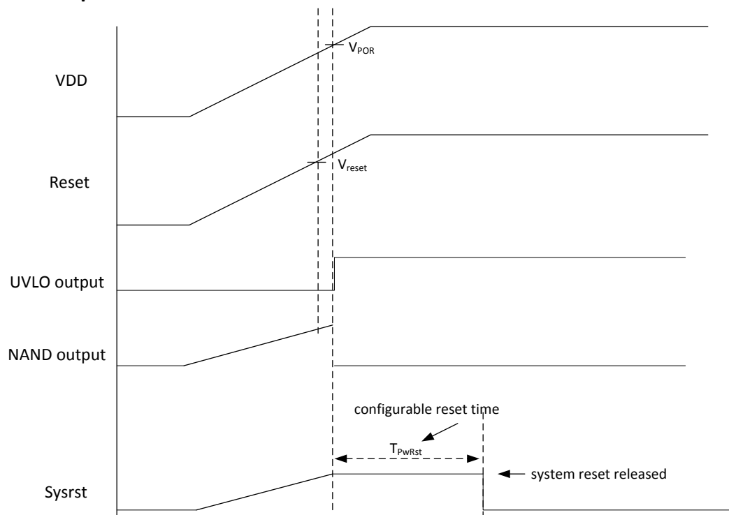
Figure 2- 4 Power-up sequence
