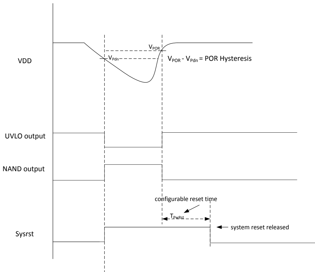
Figure 2- 5 Power-down sequence
