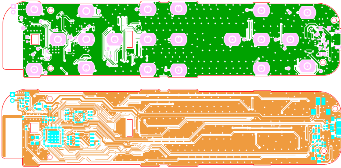
Figure 14- 2 Layout for the TLSR8267ET48 (Up: Top view; Down: Bottom view)
