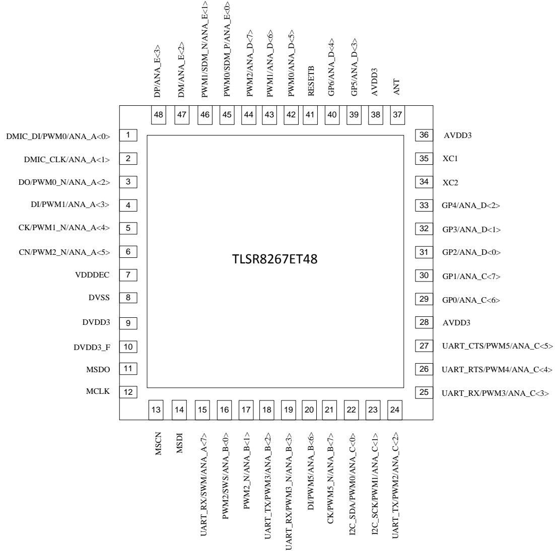
Figure 1- 5 Pin assignment for the TLSR8267ET48
