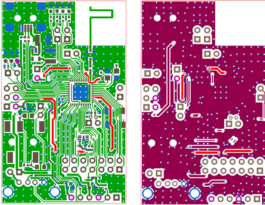
Figure 14- 4 Layout for the TLSR8267F512ET48
