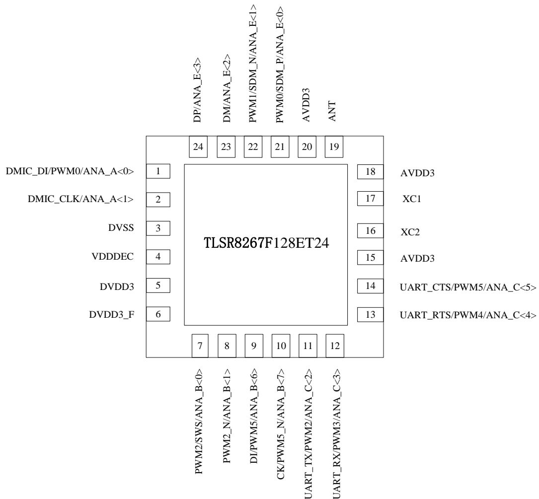
Figure 1- 8 Pin assignment for the TLSR8267F128ET24
