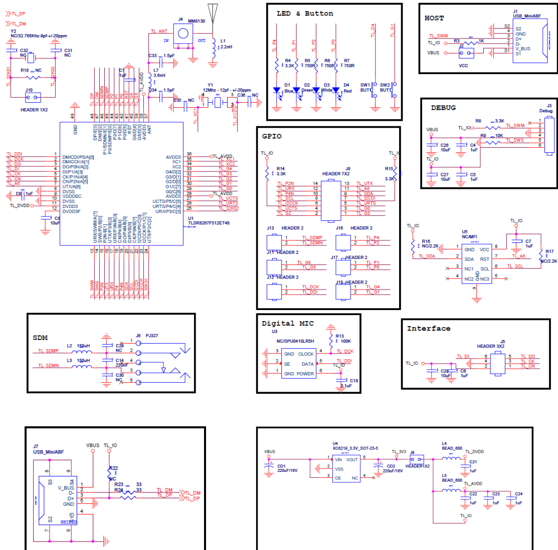
Figure 14- 3 Schematic for the TLSR8267F512ET48
