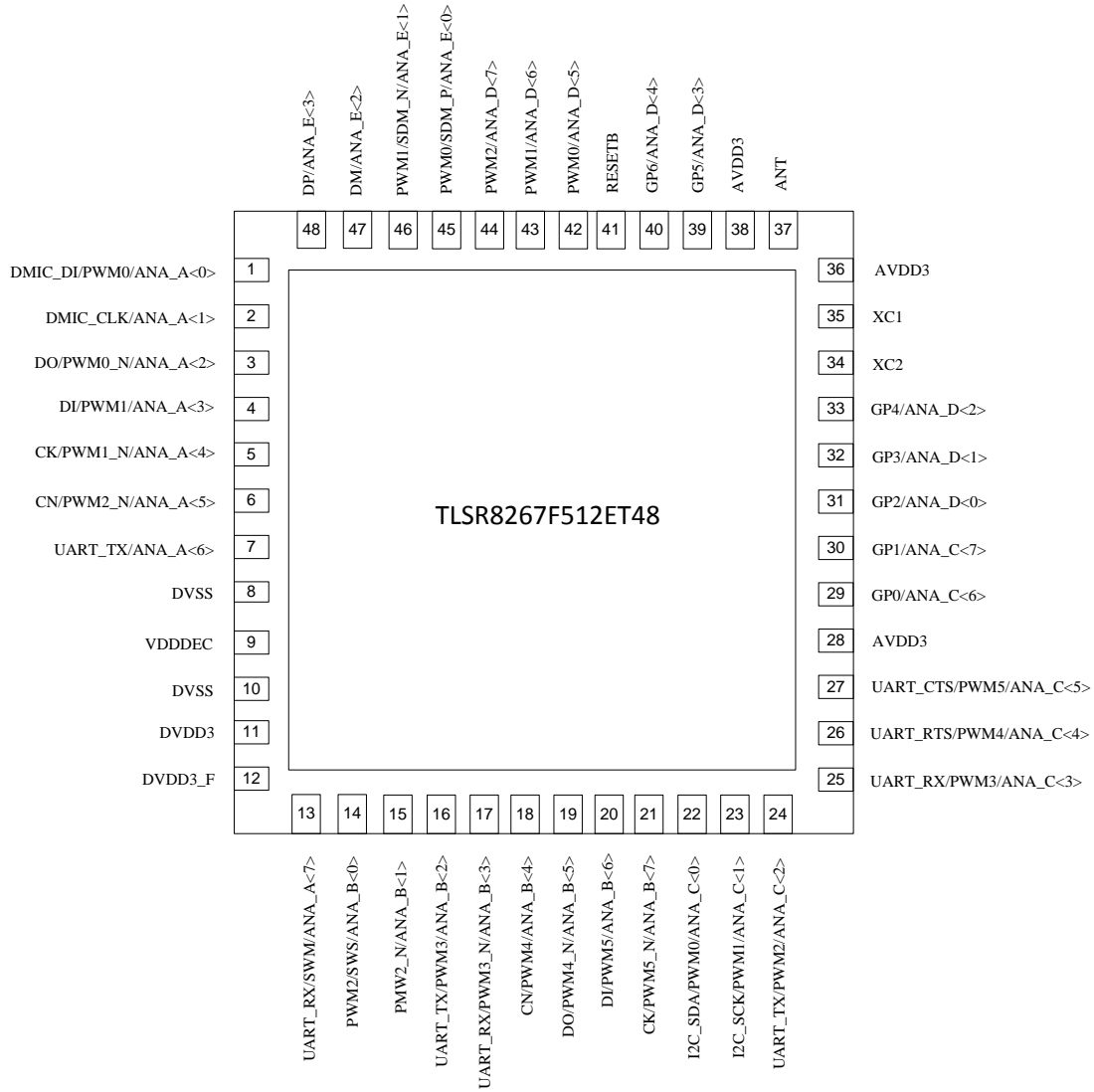
Figure 1- 6 Pin assignment for the TLSR8267F512ET48
