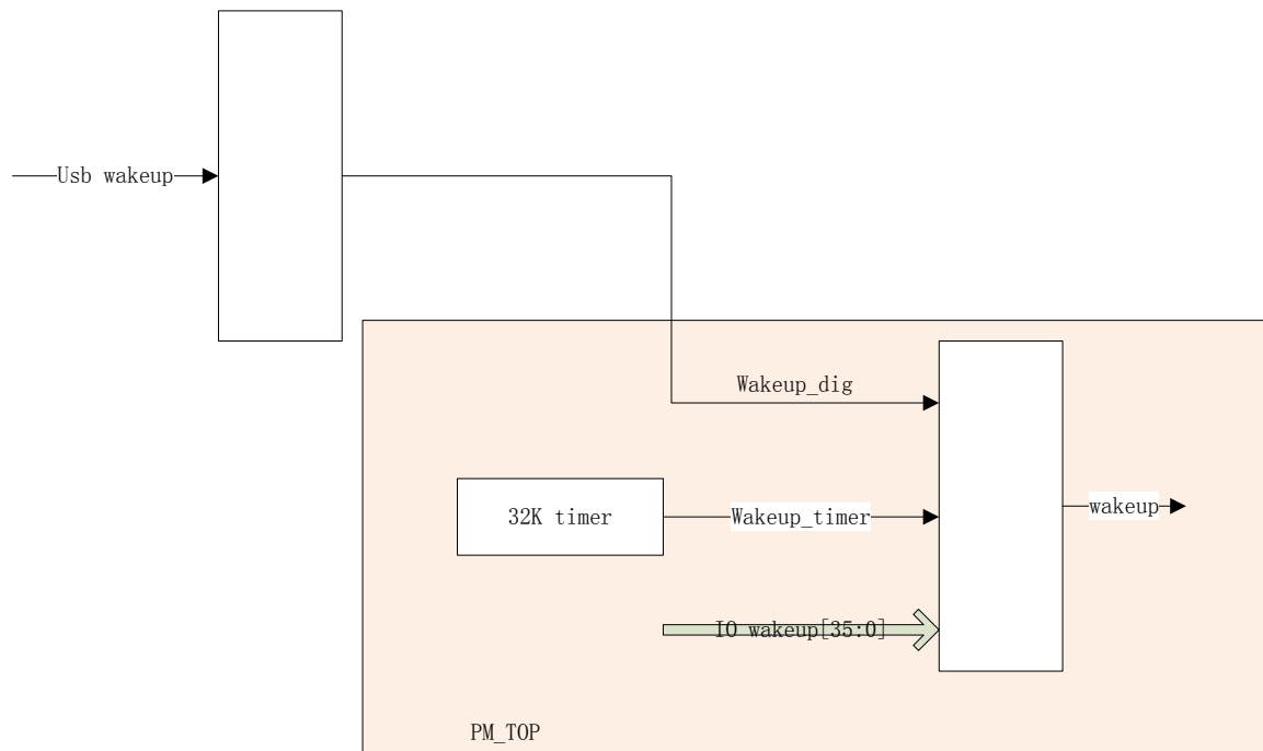
Figure 2- 6 Wakeup sources
